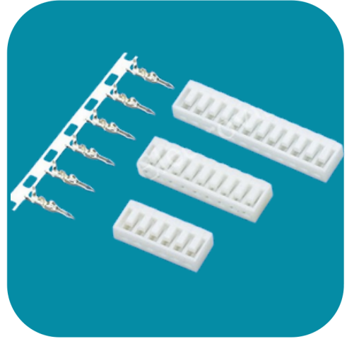
RS 255 PITCH-2.50mm
