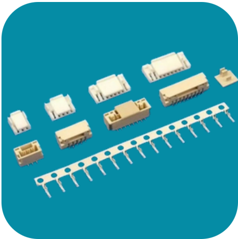
RS .... PITCH-1.25mm
