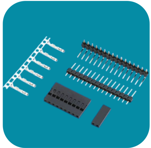
RS 257 PITCH-2.54mm
